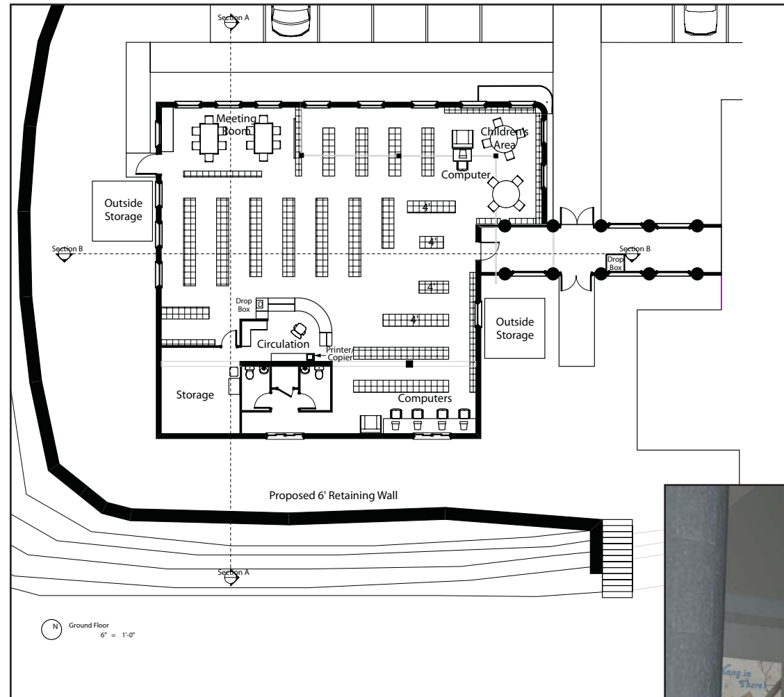
Floor and Site Plan
